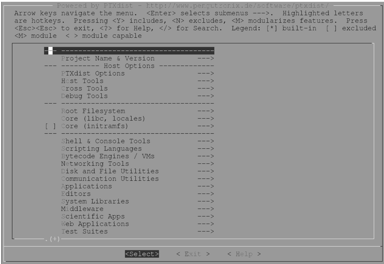
Figure 3.3: Main userland configuration menu
