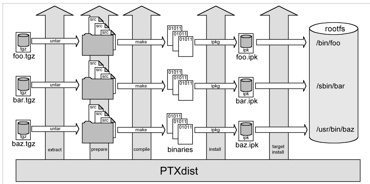
Figure 3.2: The build process
